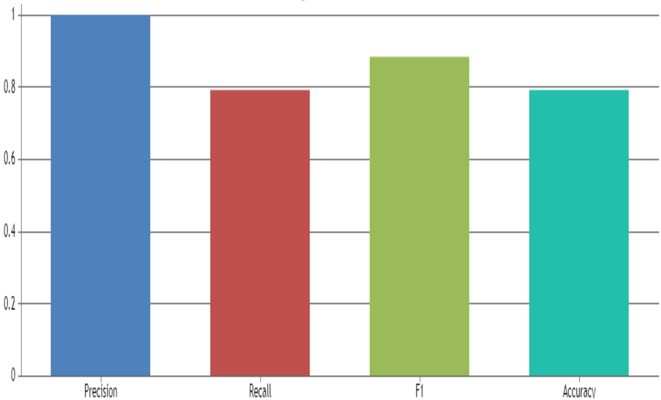
Fig. 5. Random Forest
