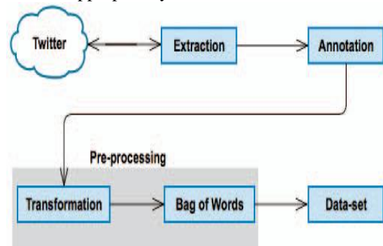
Fig. 1.Preparation of dataset
