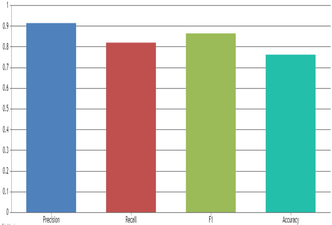
Fig. 4. Decision Tree
