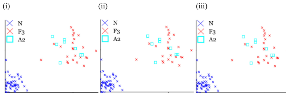
Fig. 4. Classification Results on reevaluation of NF3 model (Testbed Dataset) Fig.d, (i) Delay (ii) Throughput (iii) Delay & Throughput.
