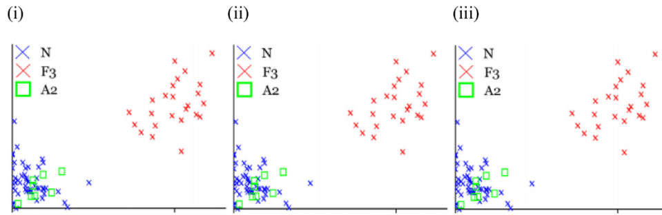
Fig. 3. Classification Results on re-evaluation of NF3 model (Simulation Dataset) Fig. 1c, with (i) SEQ feature addition (ii) Global Features Removal (iii) TOP 10 Features.
